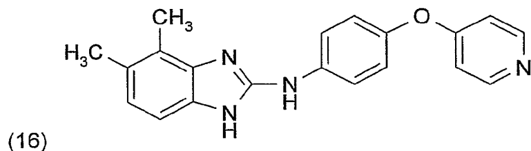
(4,5-Dimethyl-1H-benzimidazol-2-yl)-[4-(pyridin-4-yloxy)-phenyl]-amin
